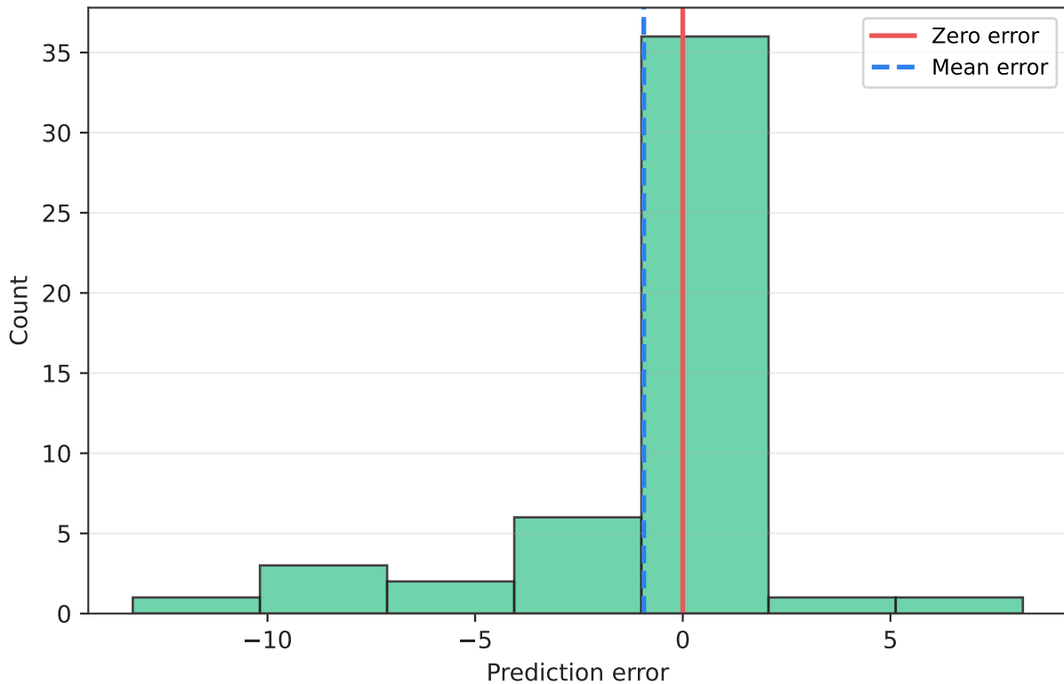
Residual Distribution: Irrigation volume
